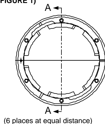
Figure 3. Latch Ring (3-Slot and 6-Slot) Detail
