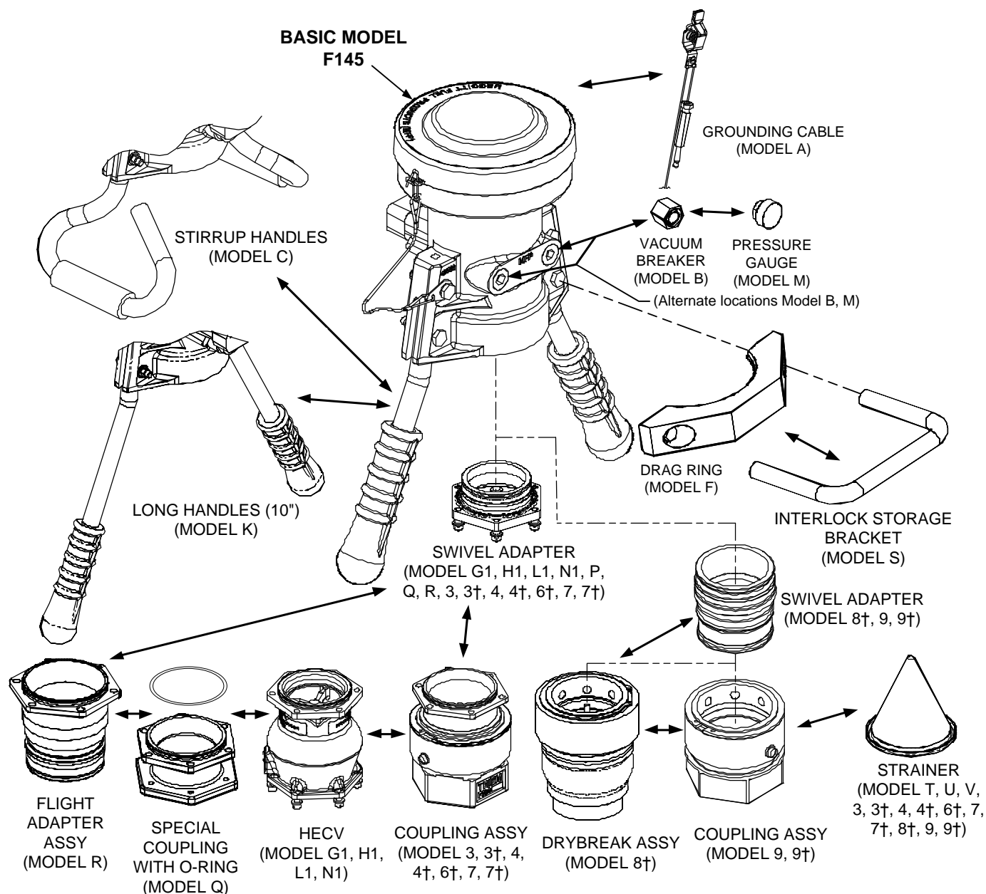
Figure 1. Pressure Fuelling Nozzle (Sheet 2)
