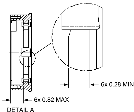
Figure 3. Latch Ring (3-Slot and 6-Slot) Detail
